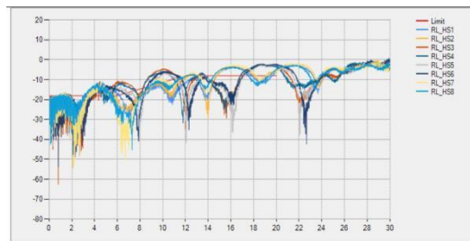
Fig.2-1 Differential Return Loss (SS Pair)
