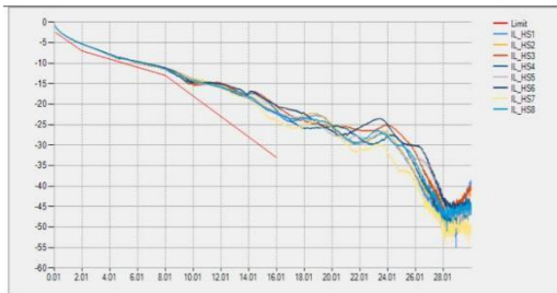
Fig.1-1 Differential Insertion Loss (SS Pair)
