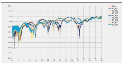
Fig.2-1 Differential Return Loss (SS Pair)
